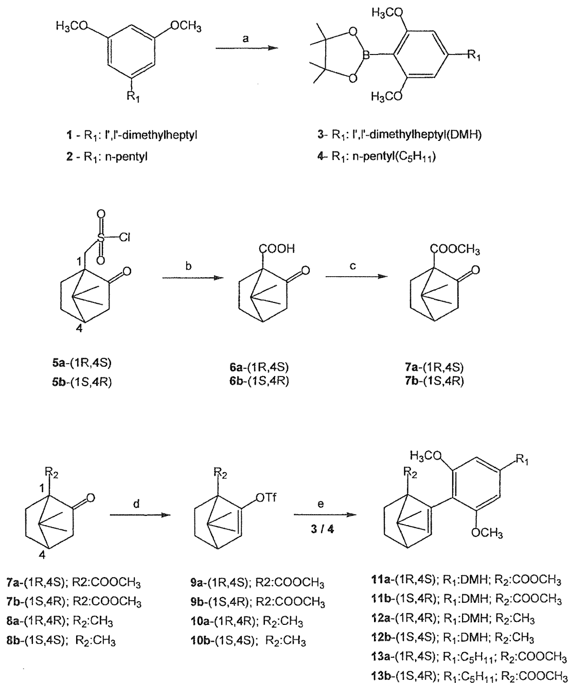
Scheme 1 a . Cross-coupling reaction at the C2-position of camphoric moiety.
