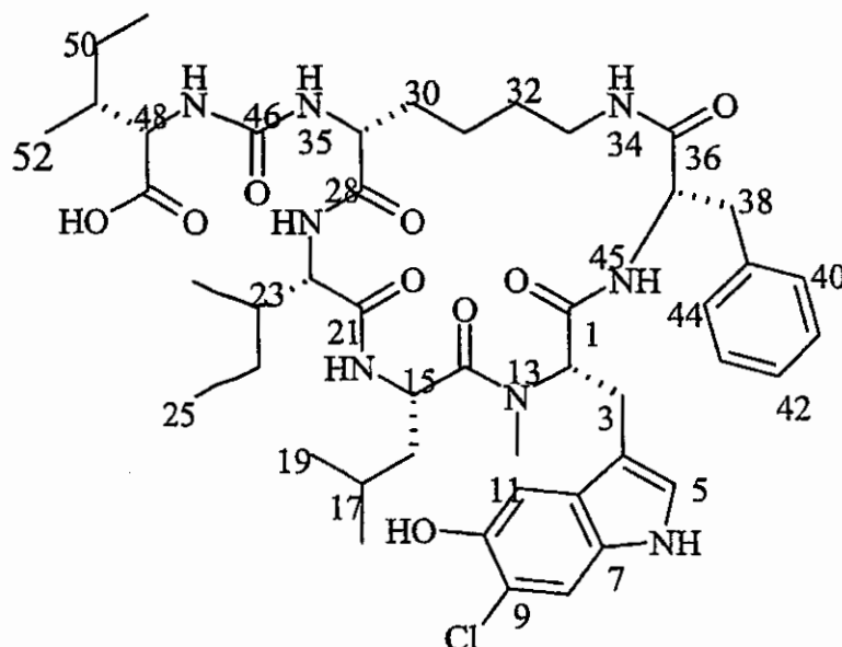
5 Table 8 1 H (600 MHz), 13 C (125 MHz) and COSY NMR data for Compound 8 in d 6 -DMSO
