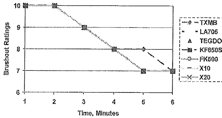
Figure 5. Acrylic Semigloss Wet Edge/Open Time Ratings
