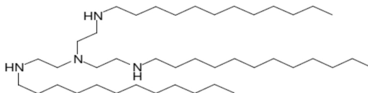
3-C12
