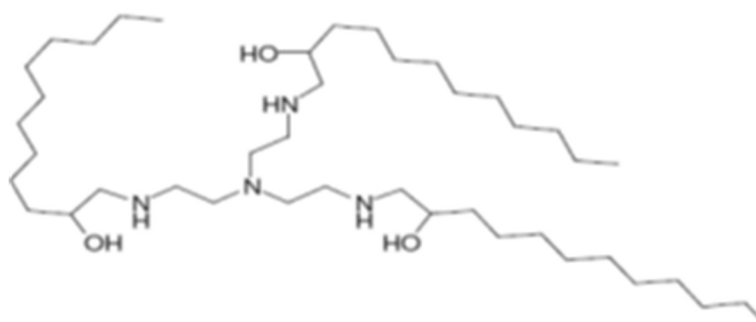
3-C12-OH
