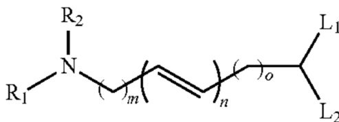
(formula III)
