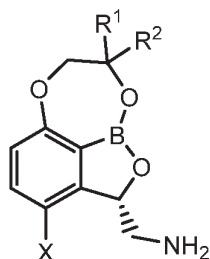
Formula IIa
