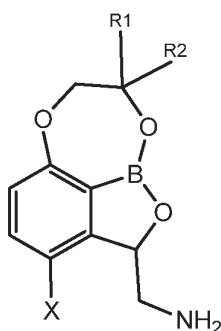
Formula II ,
