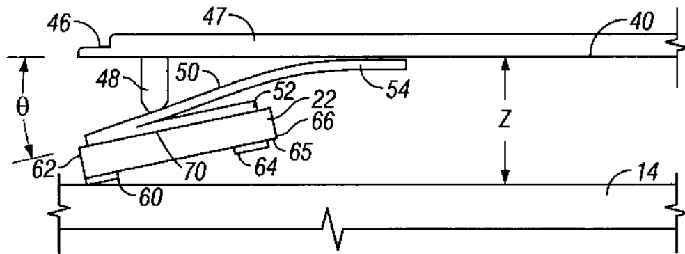
FIG. 3 (Prior Art)
