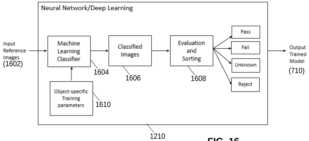
Training – Neural Network/Machine Learning
