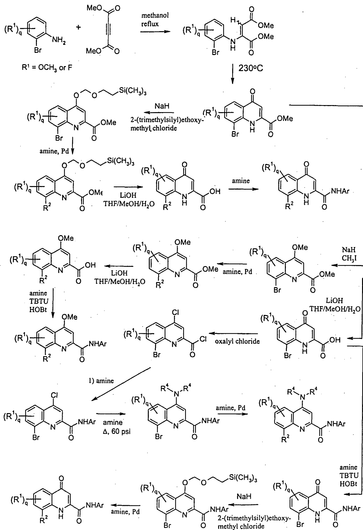
Scheme 4. Routes for preparation of quinoline and quinolone compounds of the present invention
