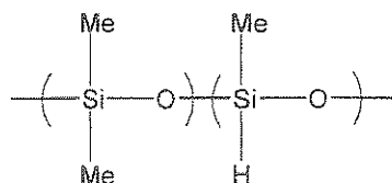
5 Scheme 3: Polymer of polysiloxane type bearing hydrosilane groups
