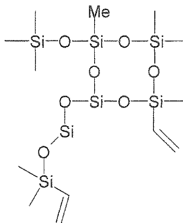
Scheme 5: VQM matrix comprising a polydimethylsiloxane micro-network
