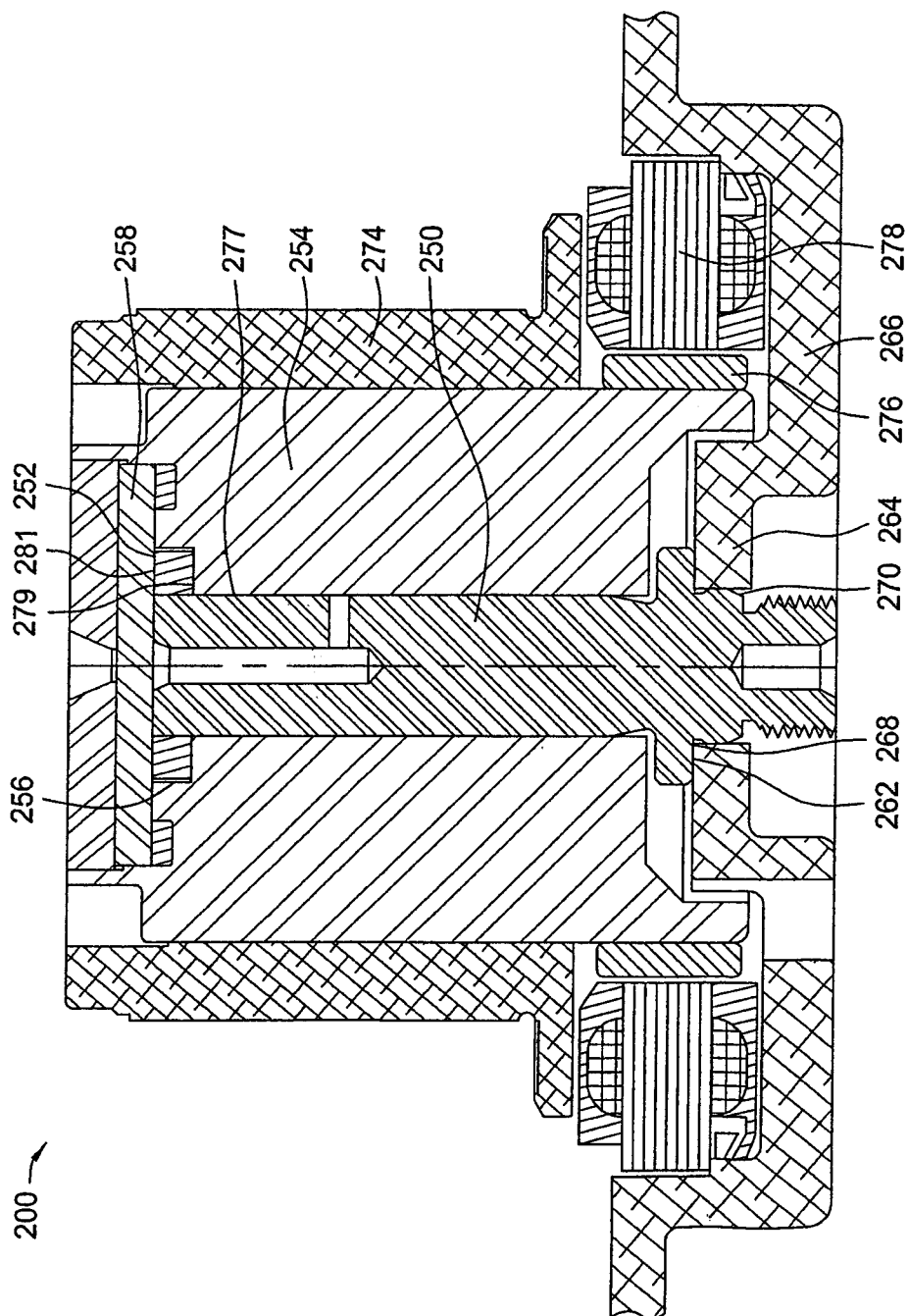
FIG. 2 (PRIOR ART)
