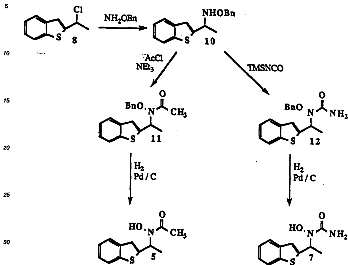
Scheme 5
