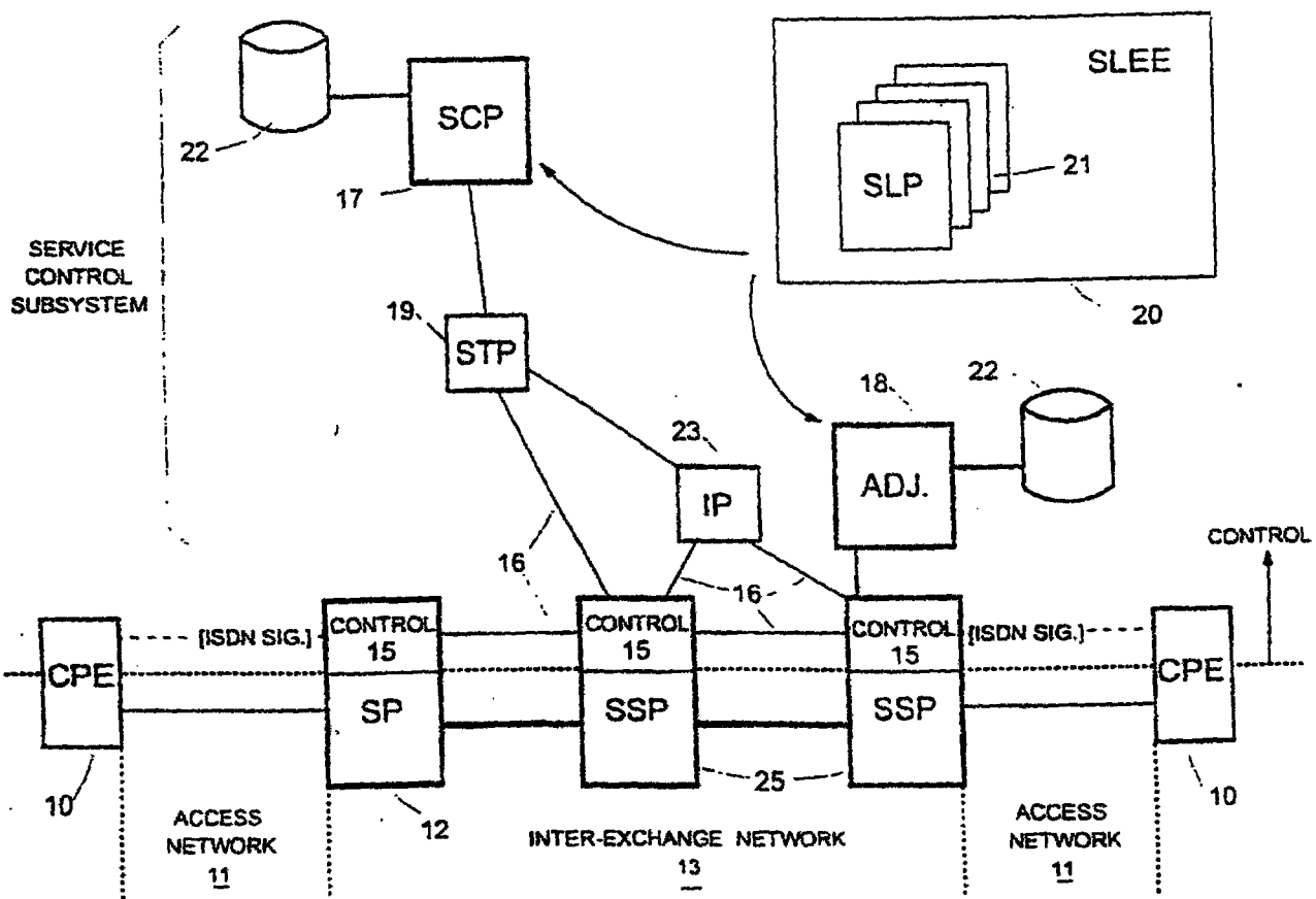
FIG. 2 (PRIOR ART)
