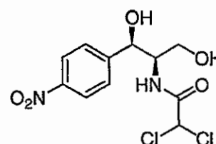
Chloramphenicol
