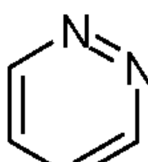
pyridazine (pyridazinyl)
