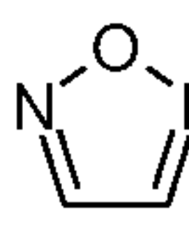
1-oxa-2,5-diazole (1-oxa-2,5-diazolyl)
