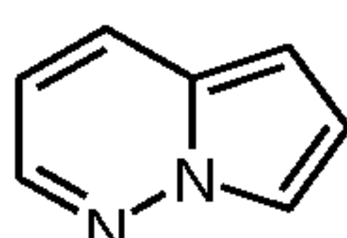
pyrrolo[1,2-b]pyridazine (pyrrolo[1,2-b]pyridazinyl)
