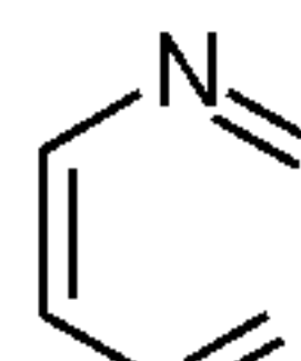
pyrimidine (pyrimidinyl)
