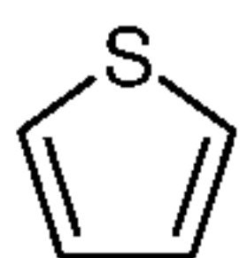
thiophene (thiophenyl)
