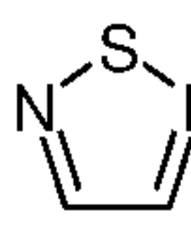
1-thia-2,5-diazole (1-thia-2,5-diazolyl)
