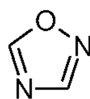
1-oxa-2,4-diazole (1-oxa-2,4-diazolyl)
