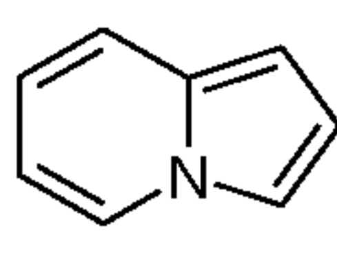
indolizine (indolinyl)
