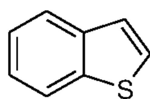
benzothiophene (benzothiophenyl)
