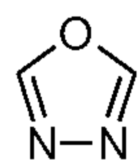
1-oxa-3,4-diazole (1-oxa-3,4-diazolyl)
