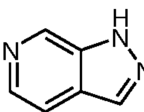
pyrazolo[3,4-c]pyridine (pyrazolo[3,4-c]pyridinyl)
