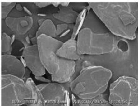
Sodium lauryl sulfate
