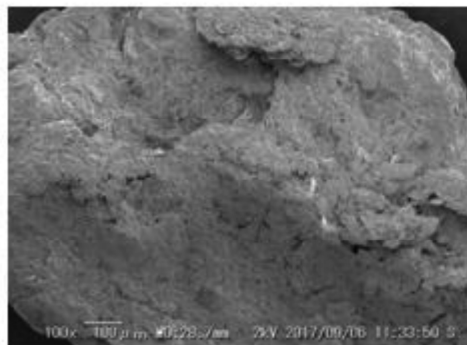
Sodium lauryl sulfate-dodecanol complex
