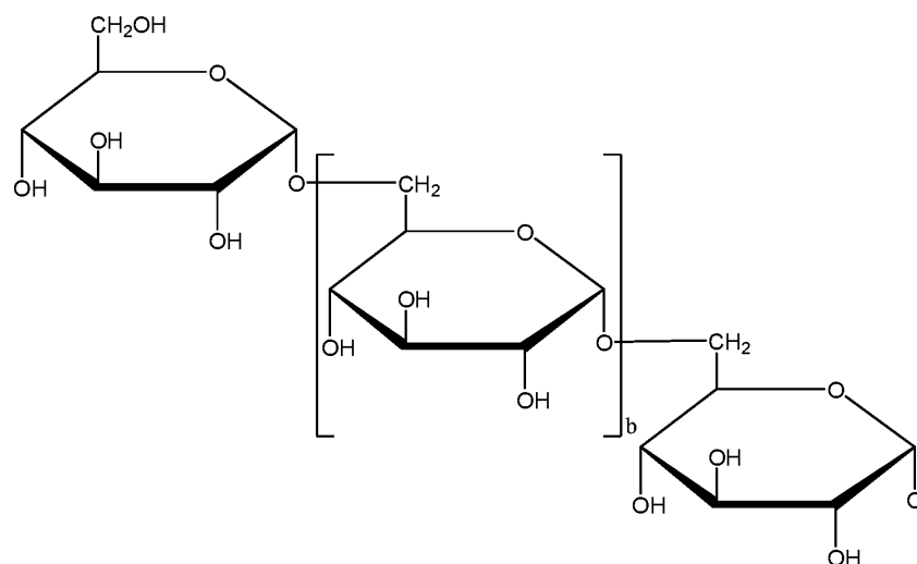
Formula 2
