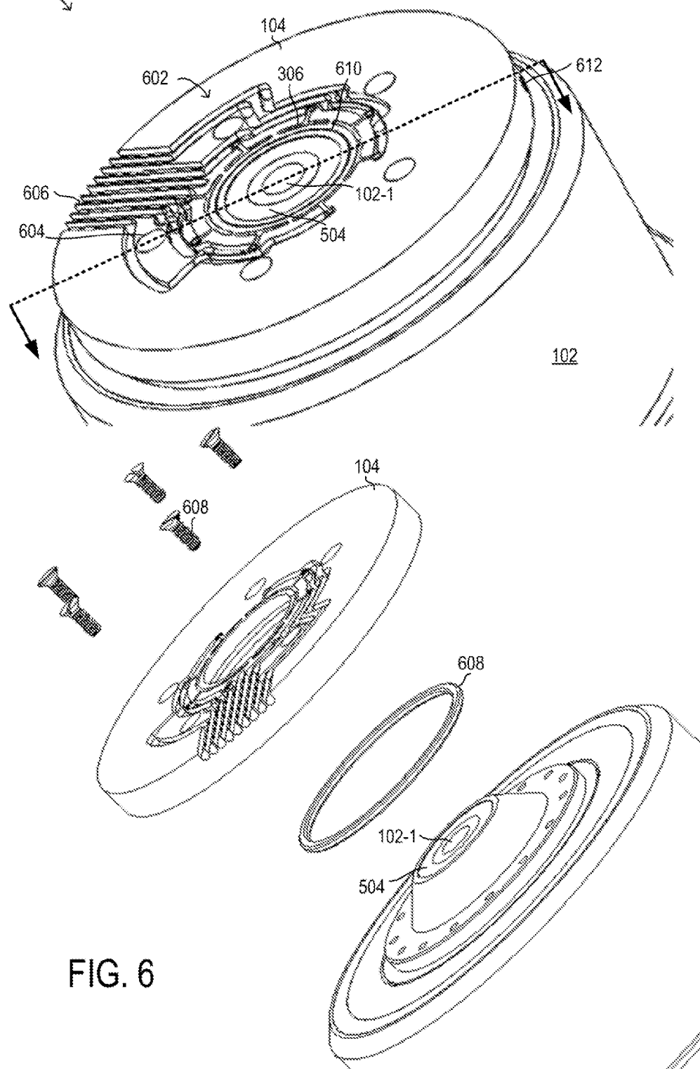
600 ASSEMBLY OF A SENSOR RING MOUNTED TO A MICROSCOPE OBJECTIVE
