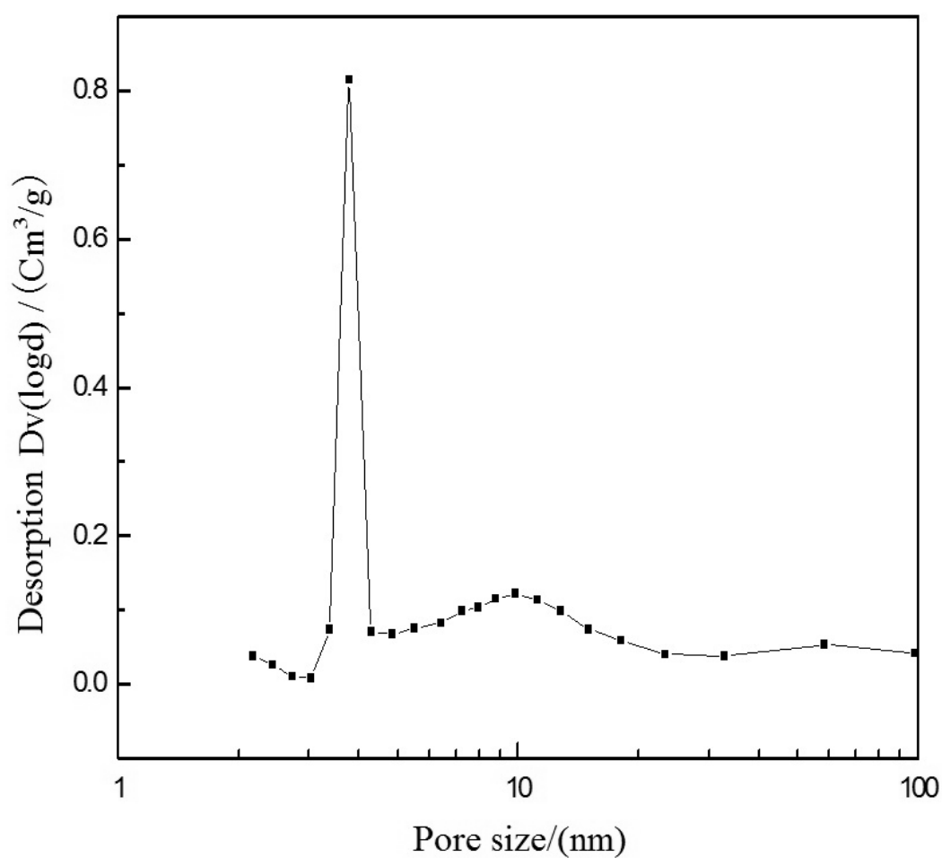
Fig. 1 Dual probable pore size distribution of the molecular sieve according to the present application
