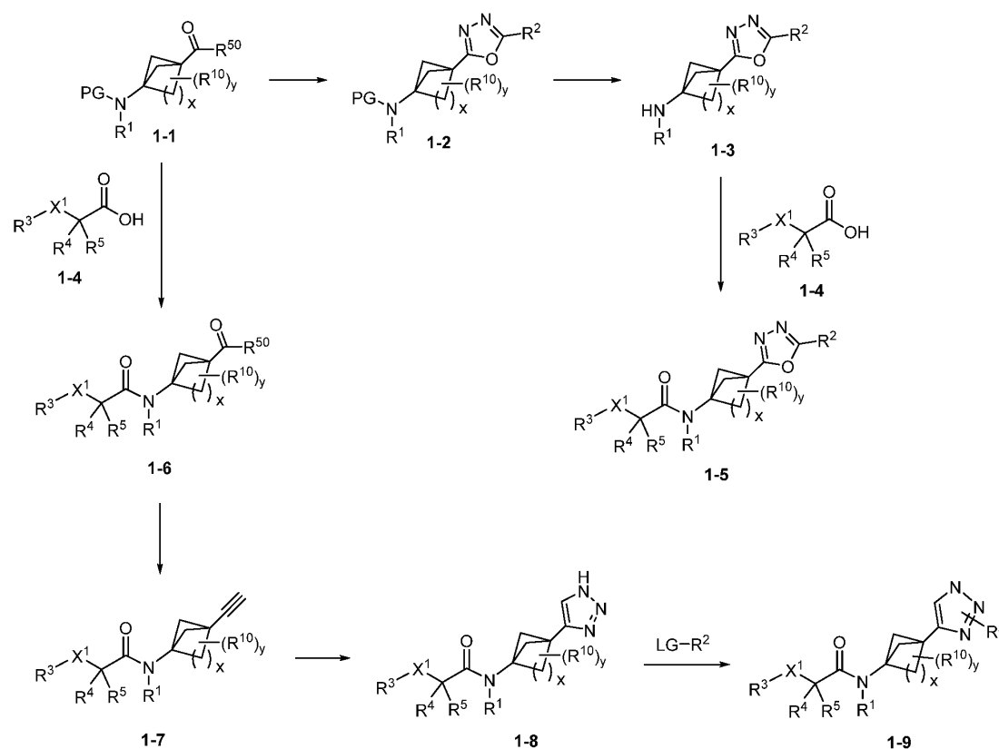
Scheme I
