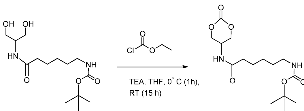
C5DHPA
