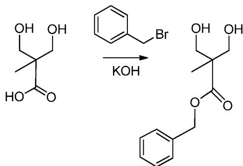
Bis-MPA
