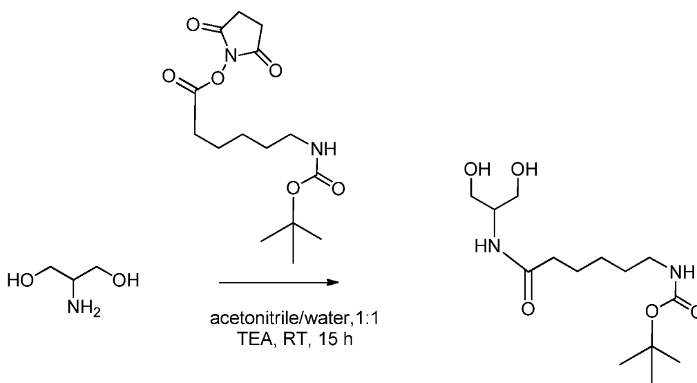
C5DHPA
