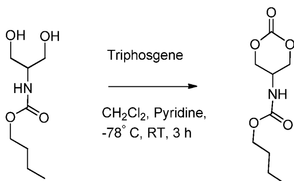
nBuDHPC
