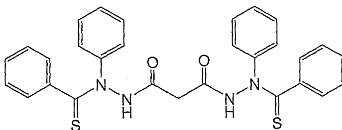
Compound (3)
