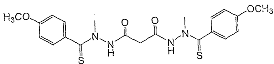
Compound (6)
