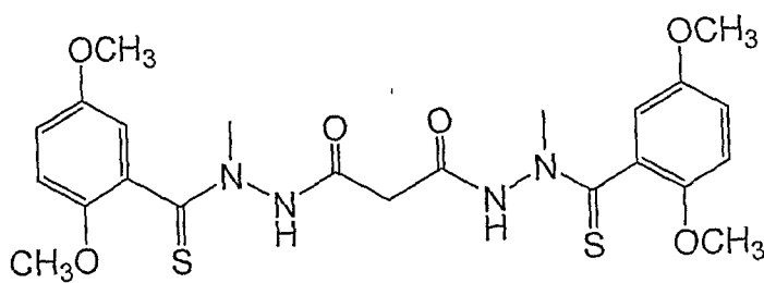
Compound (8)
