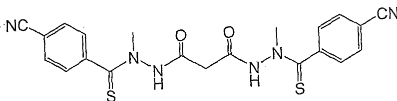
Compound (6)
