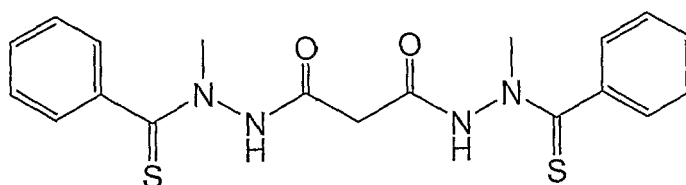
Compound (1)
