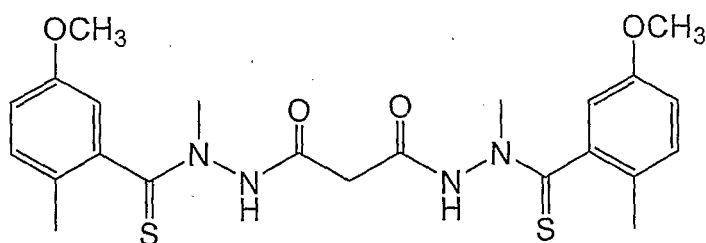
Compound (13)
