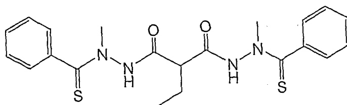
Compound (5)
