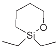
2,2-dipropyl-1-oxa-2-silacyclohexane
