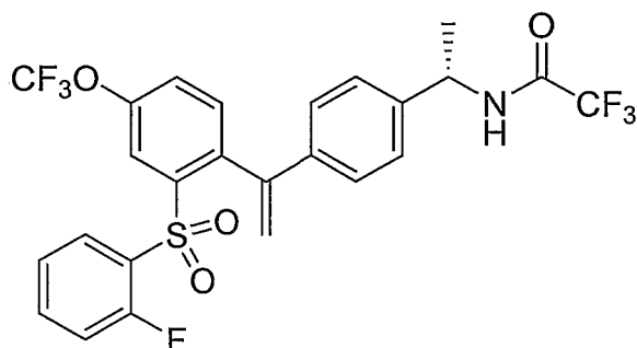
Compound 38
