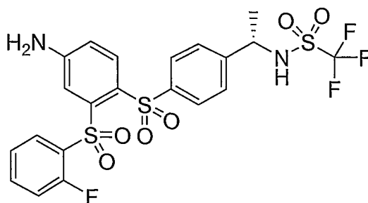
Compound XXXIII
