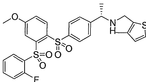
Compound XXXXXII
