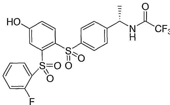
Compound 18
