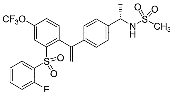
Compound XXIV
