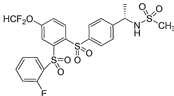
Compound XI
