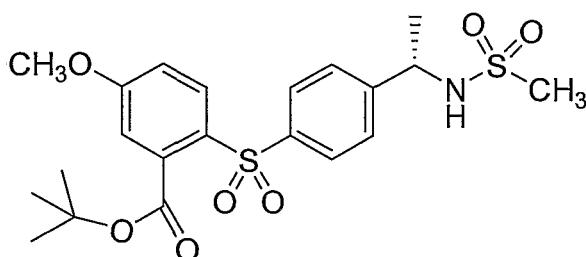
Compound XII
