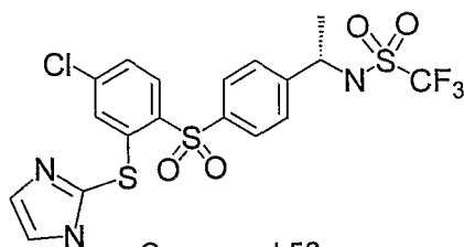
Compound 58
