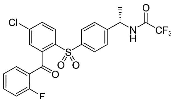
Compound 23
