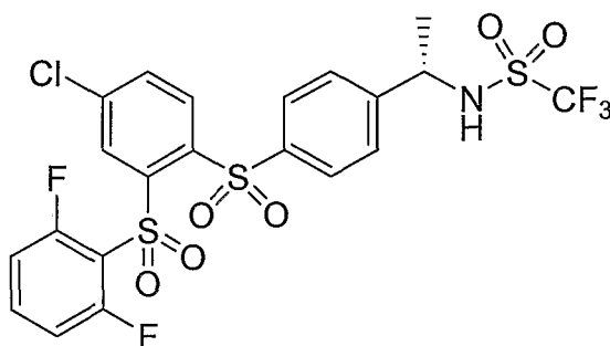
Compound VII
