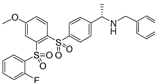
Compound XXXXXIII
