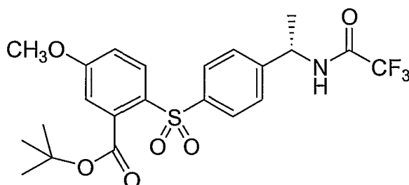
Compound 20
