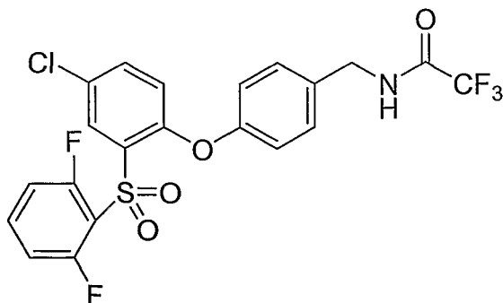
Compound 14
