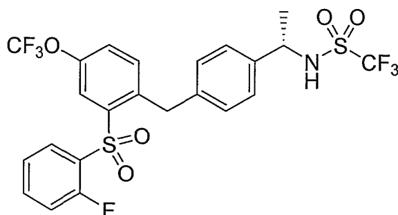
Compound XIX
