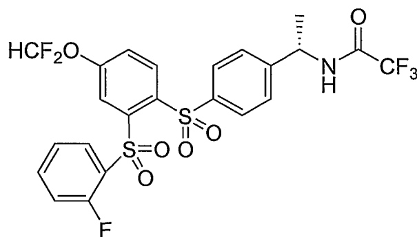
Compound 19
