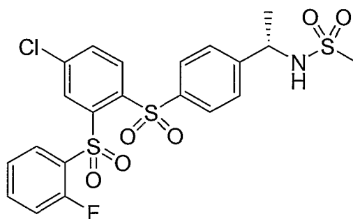
Compound IV
