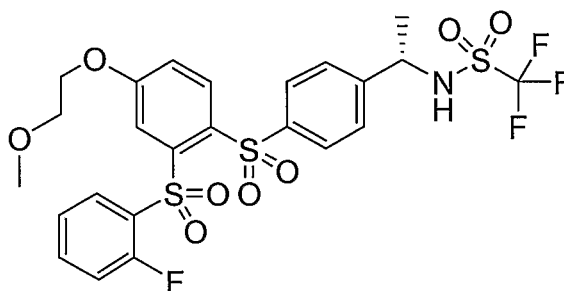
Compound XXXXV
