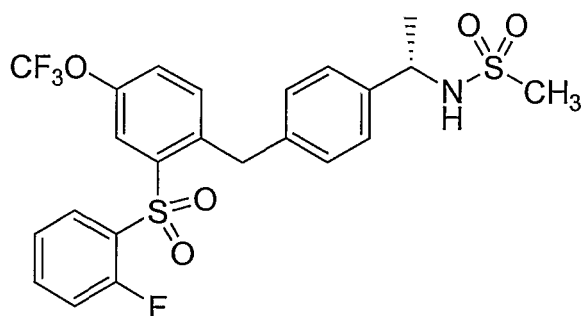
Compound 34
