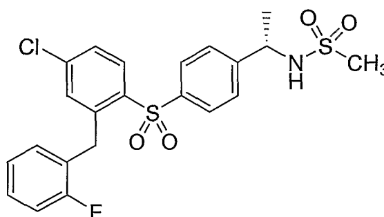
Compound XIII
