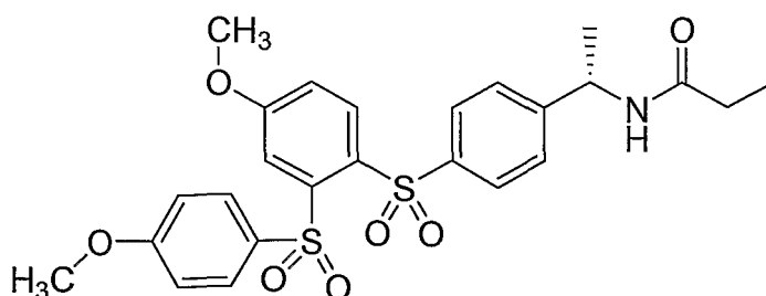
Compound II
