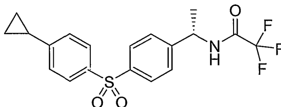
Compound 47
