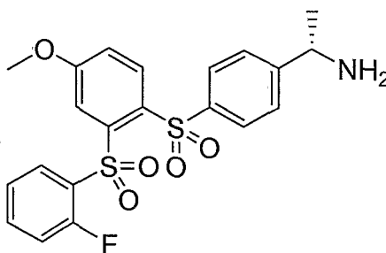
Compound 51
