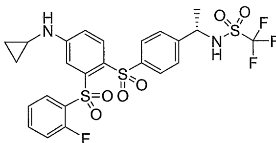
Compound XXXIV
