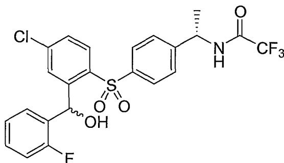
Compound 21
