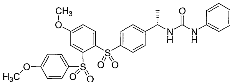
Compound III
