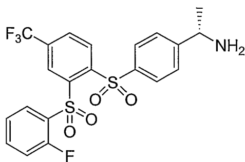
Compound 11
