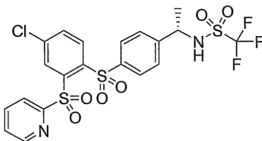
Compound XXXV
