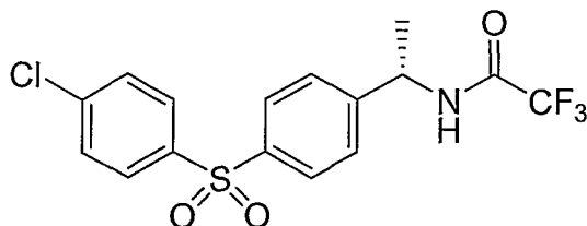
Compound 5
