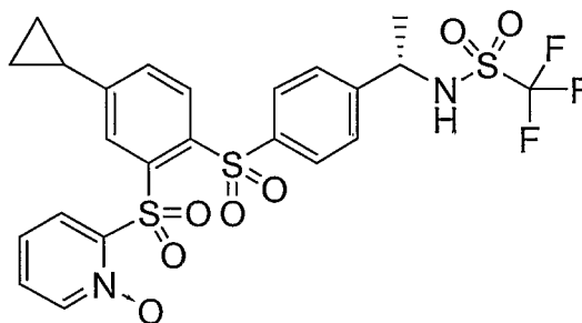
Compound XXXI
