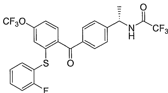
Compound 35
