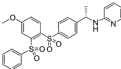
Compound XXXXXIV
