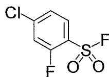
Compound 54
