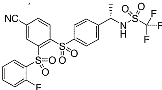
Compound XXXII
