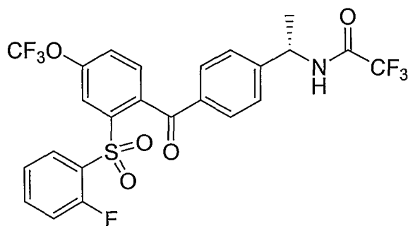
Compound 36
