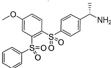
Compound 52
