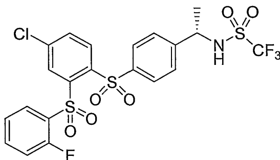
Compound V
