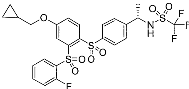
Compound XXXXIII
