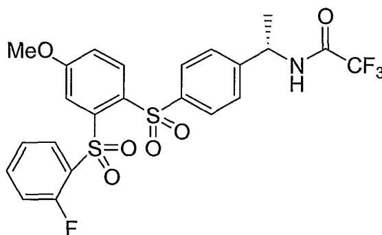
Compound 17
