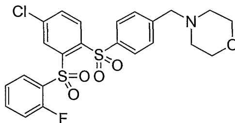
Compound XXXXX
