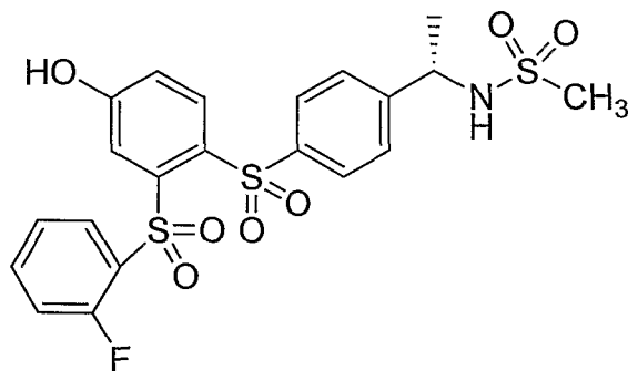
Compound X
