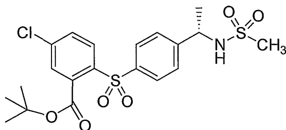
Compound 25
