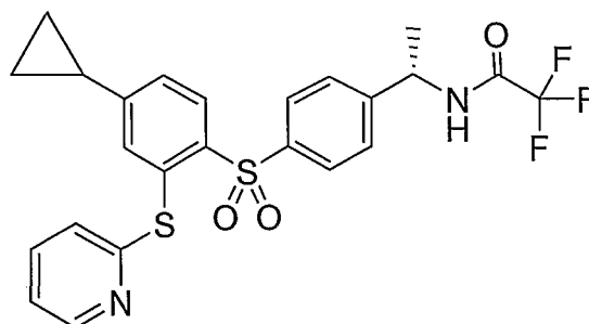
Compound 48
