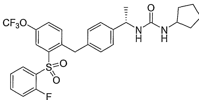
Compound XXII
