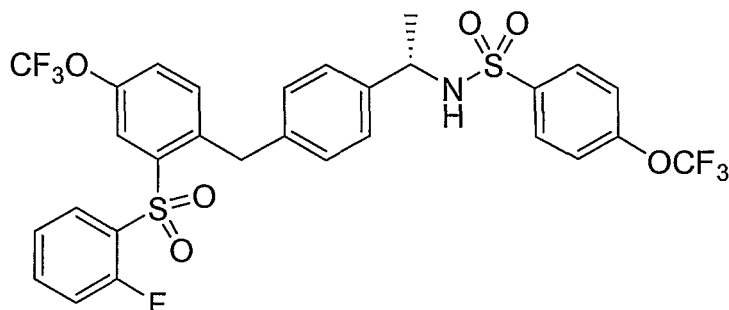
Compound XX
