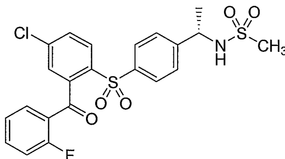
Compound XIV
