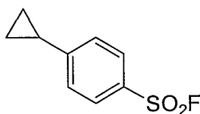
Compound 46
