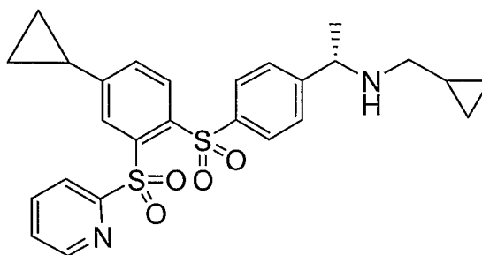
Compound XXXXIX
