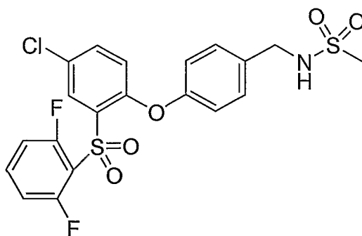
Compound IX
