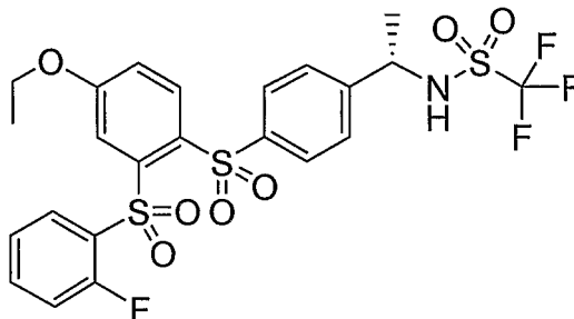
Compound XXXXIV
