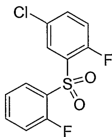
Compound 41
