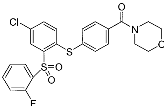
Compound XXVII
