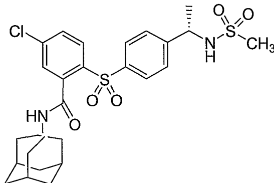
Compound XVI
