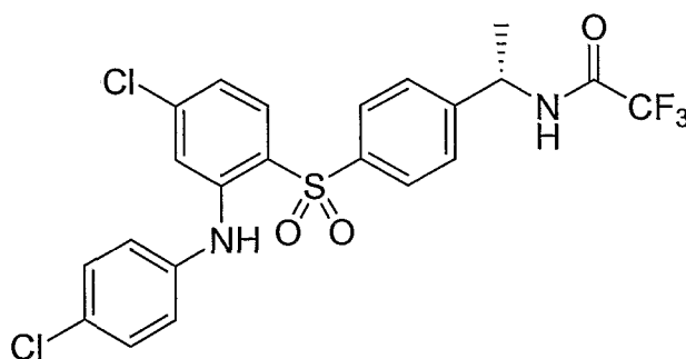
Compound 27
