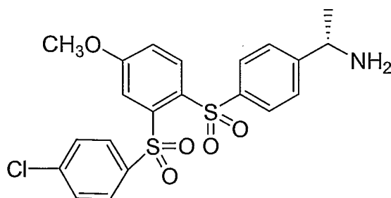
Compound 40
