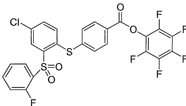
Compound 43
