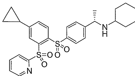
Compound XXXXVIII
