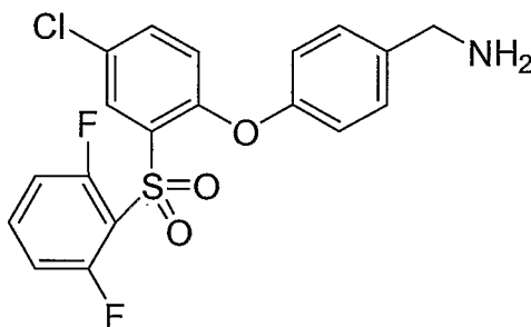
Compound 15
