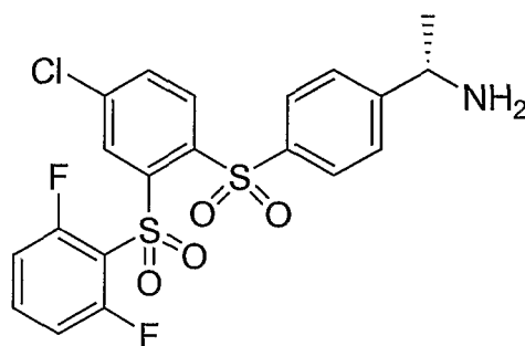
Compound 9
