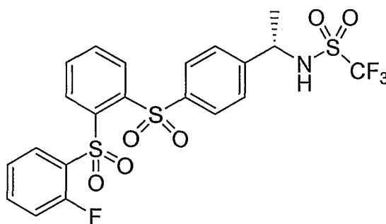
Compound VI
