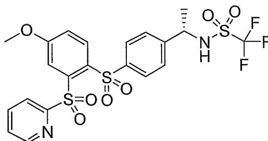
Compound XXXXXV
