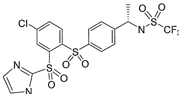
Compound XXXXXVII
