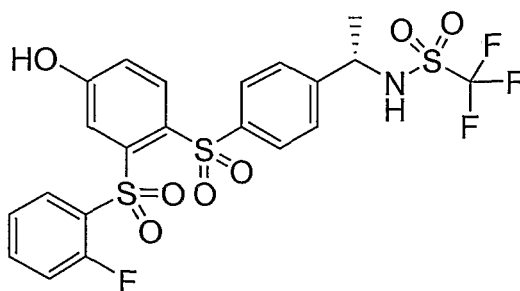
Compound XXXXI
