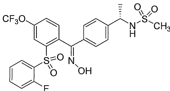
Compound XXV
