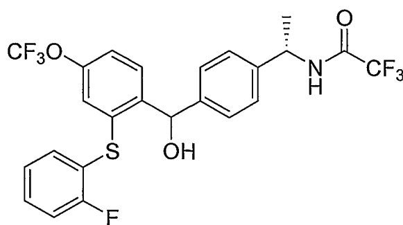
Compound 30
