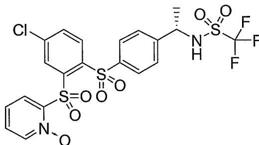
Compound XXXVI
