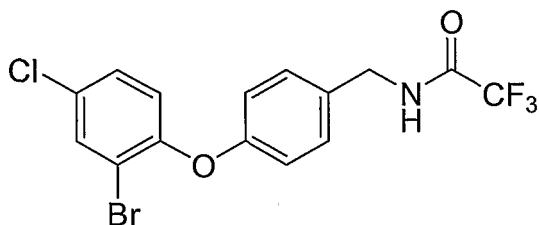
Compound 13
