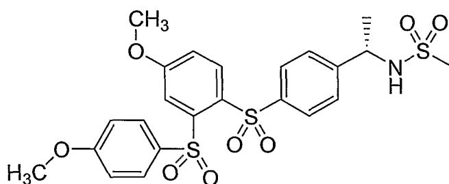
Compound I
