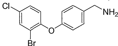
Compound 12
