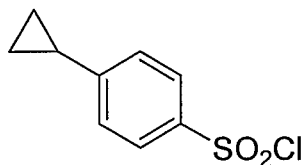
Compound 45
