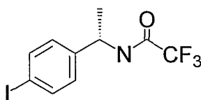
Compound 55
