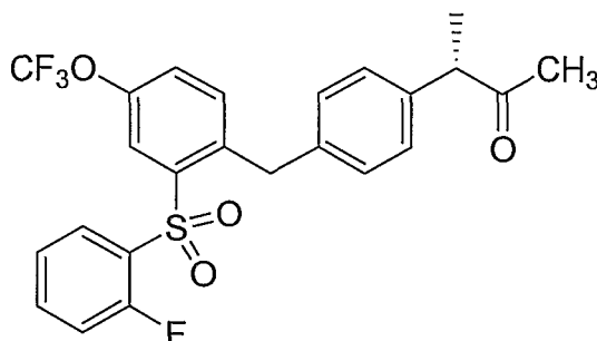
Compound XXI
