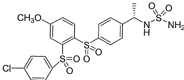
Compound XXVI
