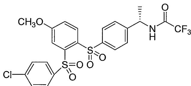
Compound 39
