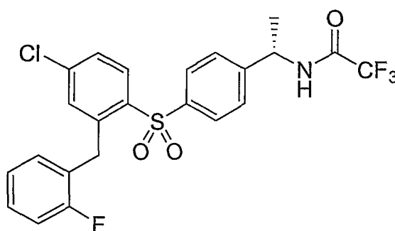
Compound 22
