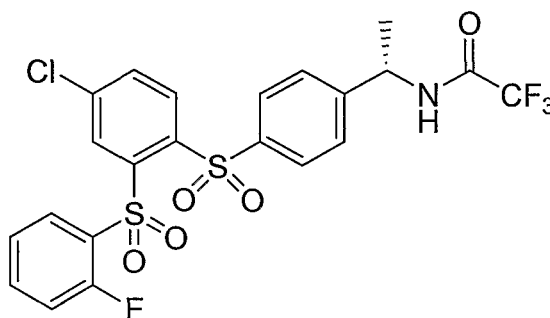
Compound 6
