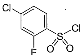
Compound 53
