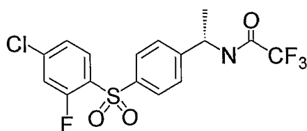
Compound 56
