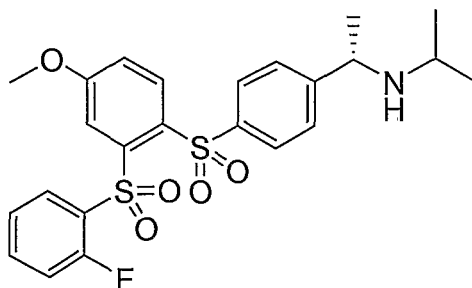
Compound XXXXXI
