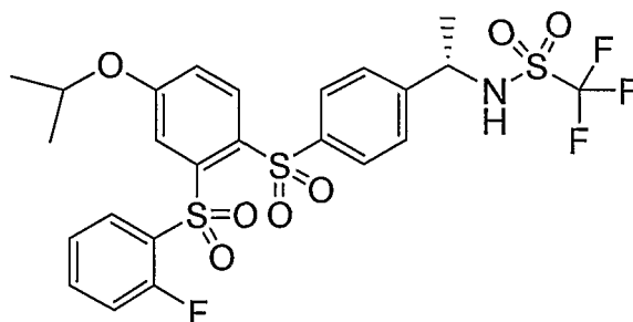
Compound XXXXII
