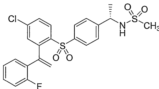
Compound XV
