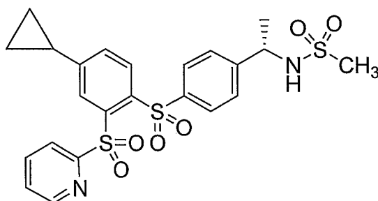
Compound XXXXXVI
