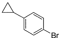
Compound 44
