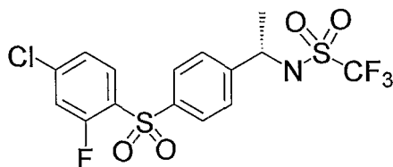
Compound 57
