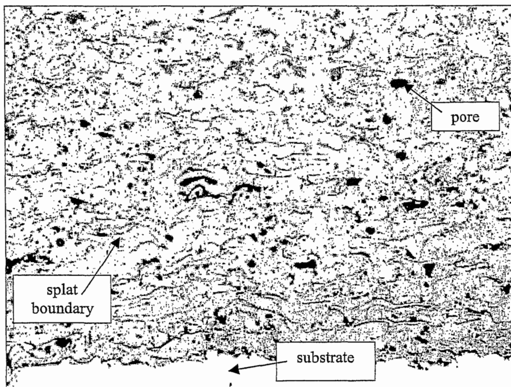
Pre-alloyed YSZ coating B 11.0% Porosity 200x
