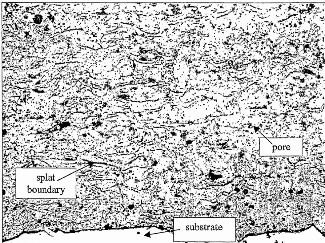
Pre-alloyed YSZ coating A 11.8% Porosity 200x
