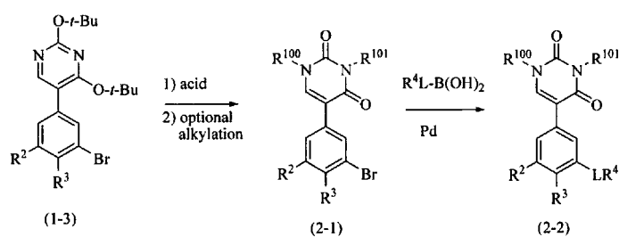
Scheme 2
