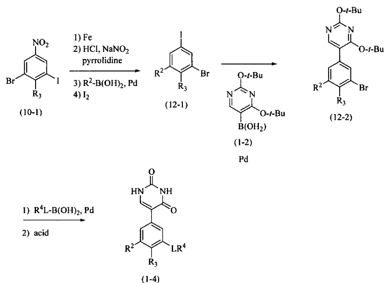
Scheme 12
