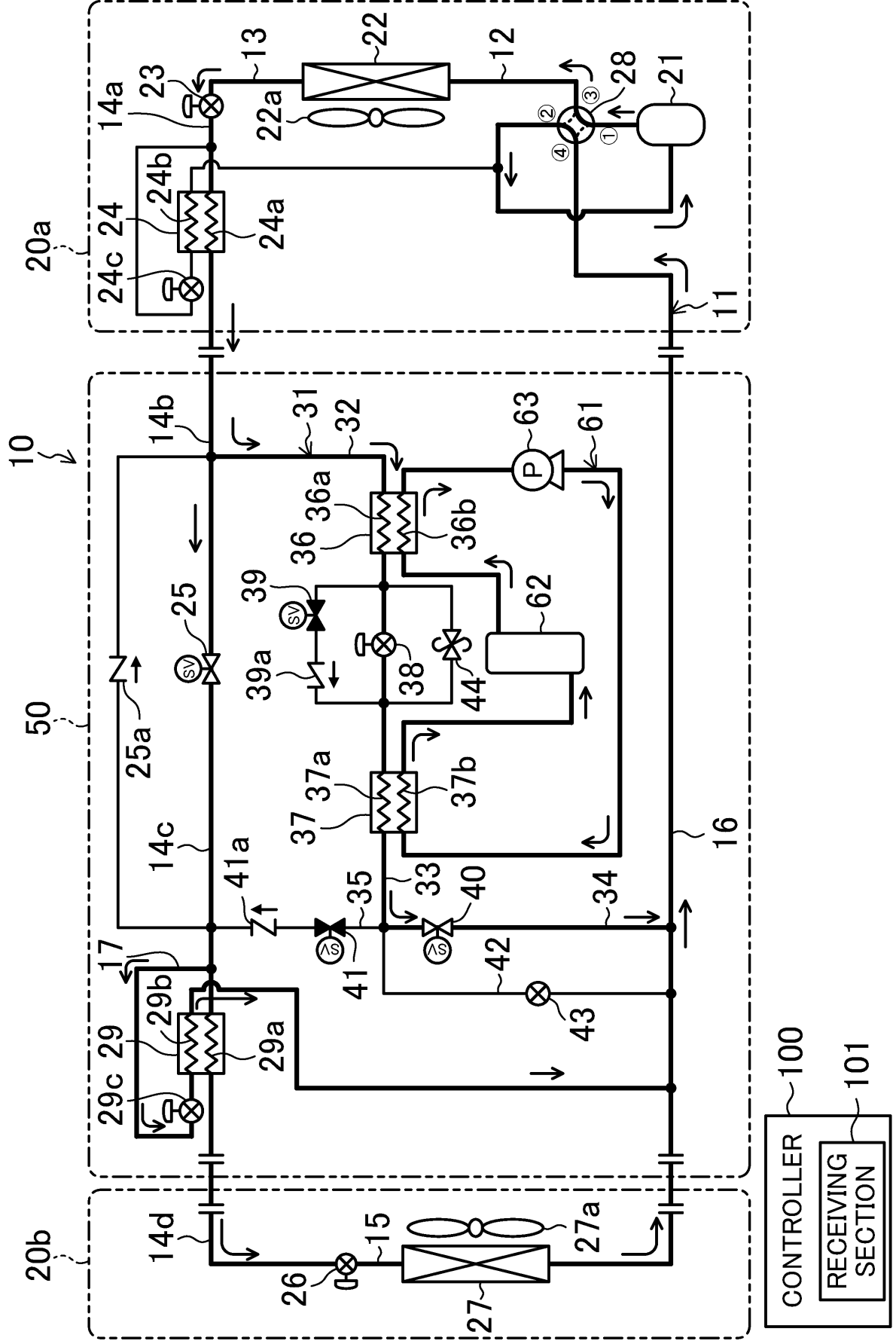
FIG.6 COOLING AND COLD THERMAL ENERGY STORAGE OPERATION
