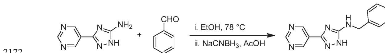
Intermediate 22
