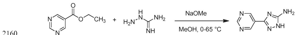
Intermediate 20
