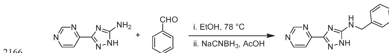
Intermediate 21
