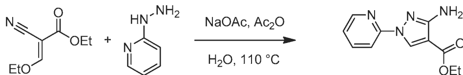
Intermediate 32
