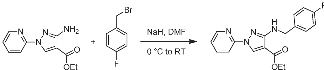
Intermediate 33
