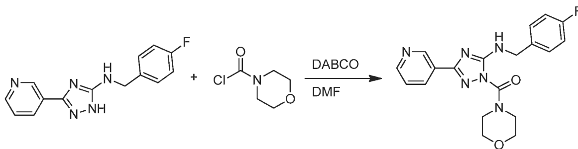
Intermediate 6
