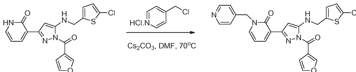
Compound 4
