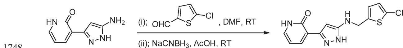
Compound 1
