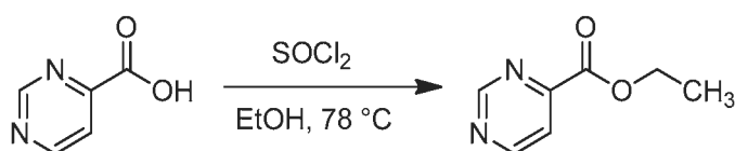
Intermediate 19
