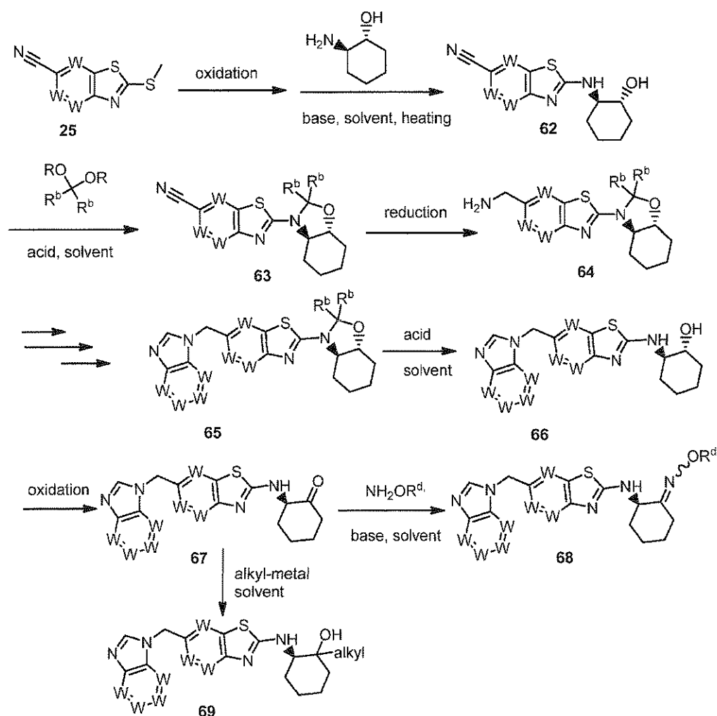
Scheme 10: General synthesis of compounds of formula (I).
