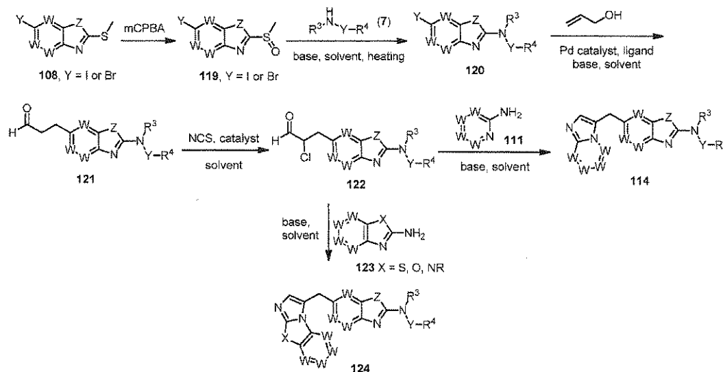
Scheme 20: General synthesis of compounds of formula (I).
