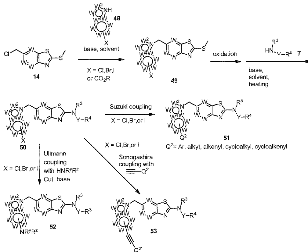
Scheme 7: General synthesis of compounds of formula (I).
