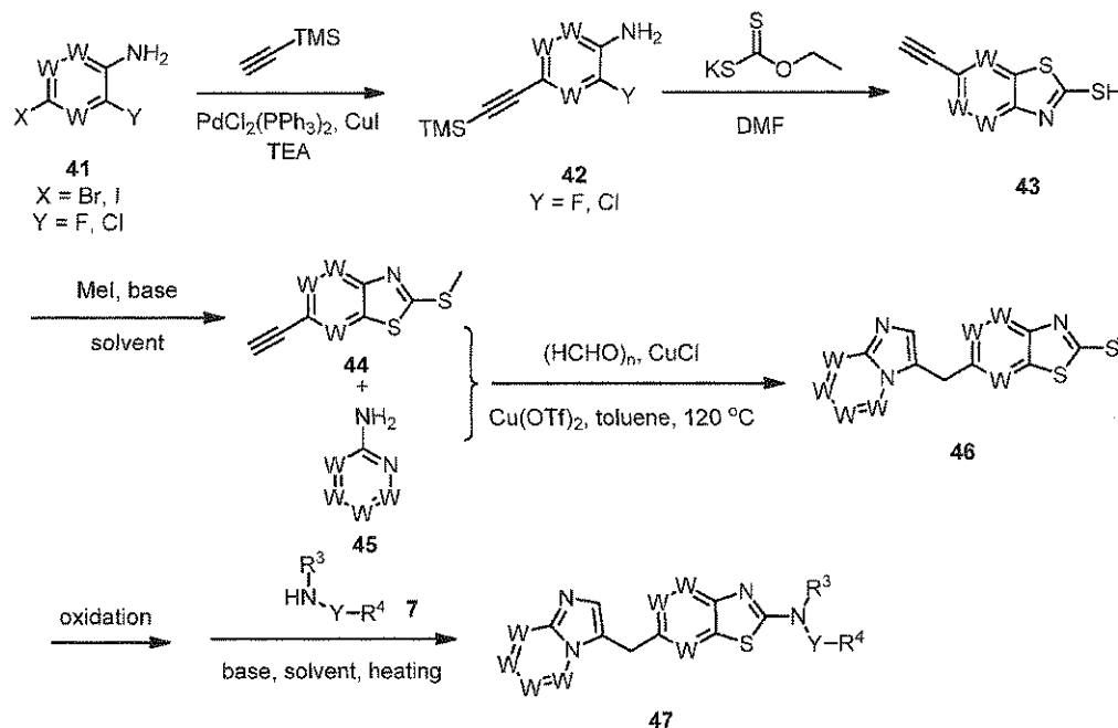
Scheme 6: General synthesis of compounds of formula (I).
