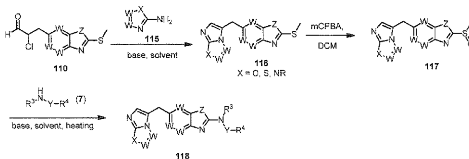
Scheme 19: General synthesis of compounds of formula (I).
