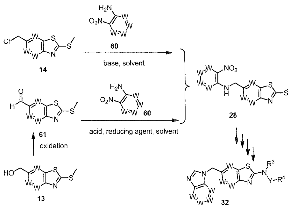
Scheme 9: General synthesis of compounds of formula (I).
