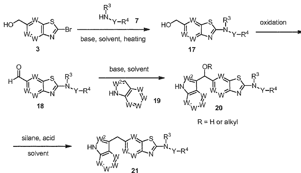
Scheme 3: General synthesis of compounds of formula (I).
