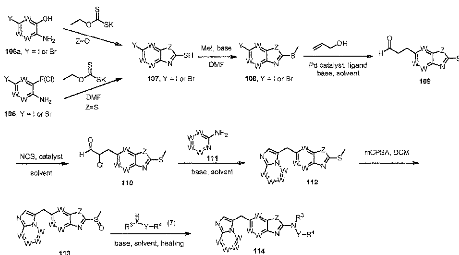
Scheme 18: General synthesis of compounds of formula (I).
