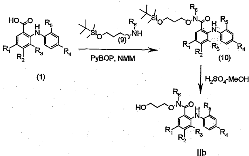
Scheme 5: Representative Preparation of Hydroxylated Benzamides Using a Silyl Ether as a Hydroxyl Protecting Group
