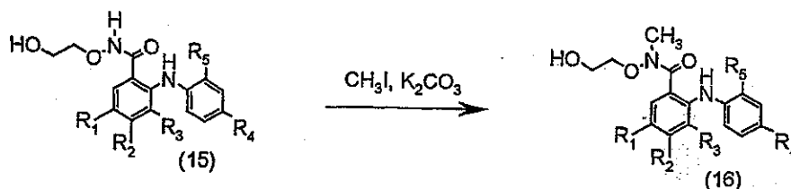
Scheme 8: Representative Preparation of Tertiary Benzamides by N-Alkylation
