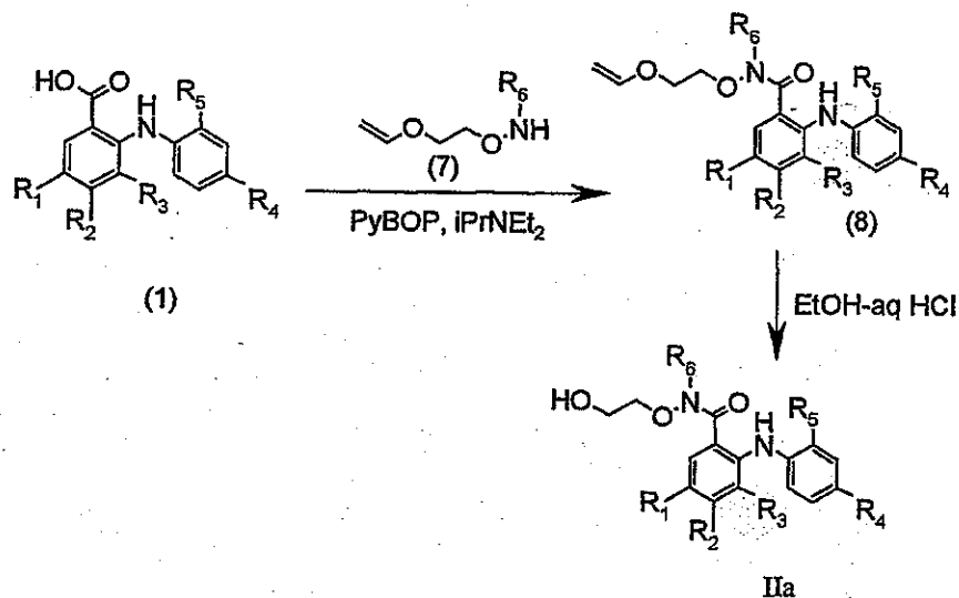
Scheme 4: Representative Preparation of Hydroxylated Benzamides Using a Vinyl Ether as a Hydroxyl Protecting Group
