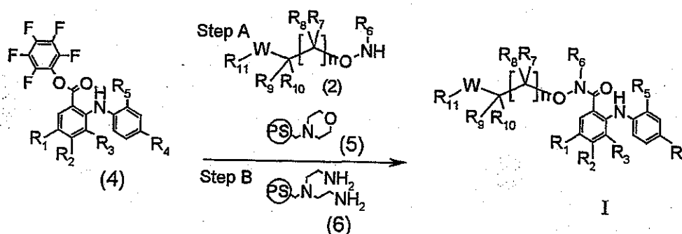
Scheme 3: General Combinatorial Preparation of Benzamides from Benzoic Acid Pentafluorophenyl Esters
