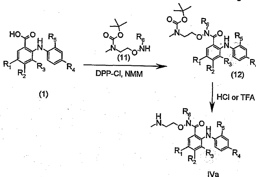
Scheme 6: Representative Preparation of Amino-Substituted Benzamides Using a tert-Butyl Carbamate as an Amino Protecting Group
