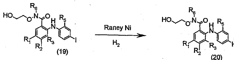
Scheme 10: Representative Hydrogenolysis of Aryl Iodides
