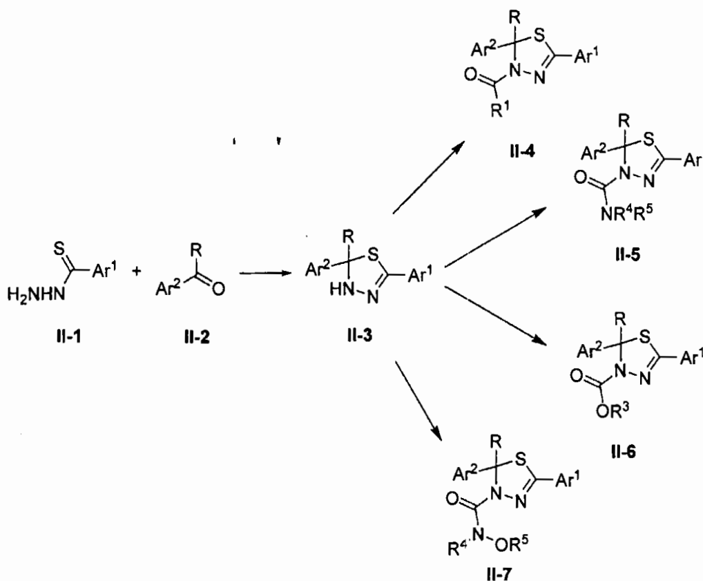
Scheme II
