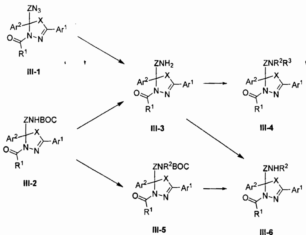
Scheme III
