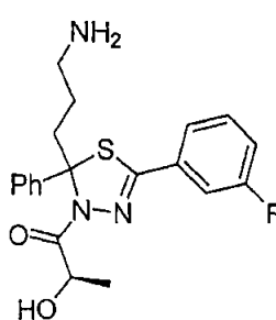
(Diastereomer B)
