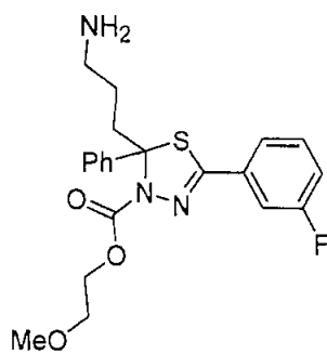
(Diastereomer B)
