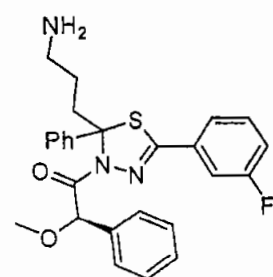
(Diastereomer B)
