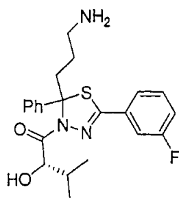
(Diastereomer B)
