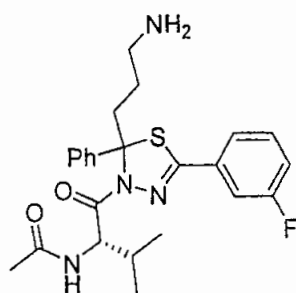
(Diastereomer B)
