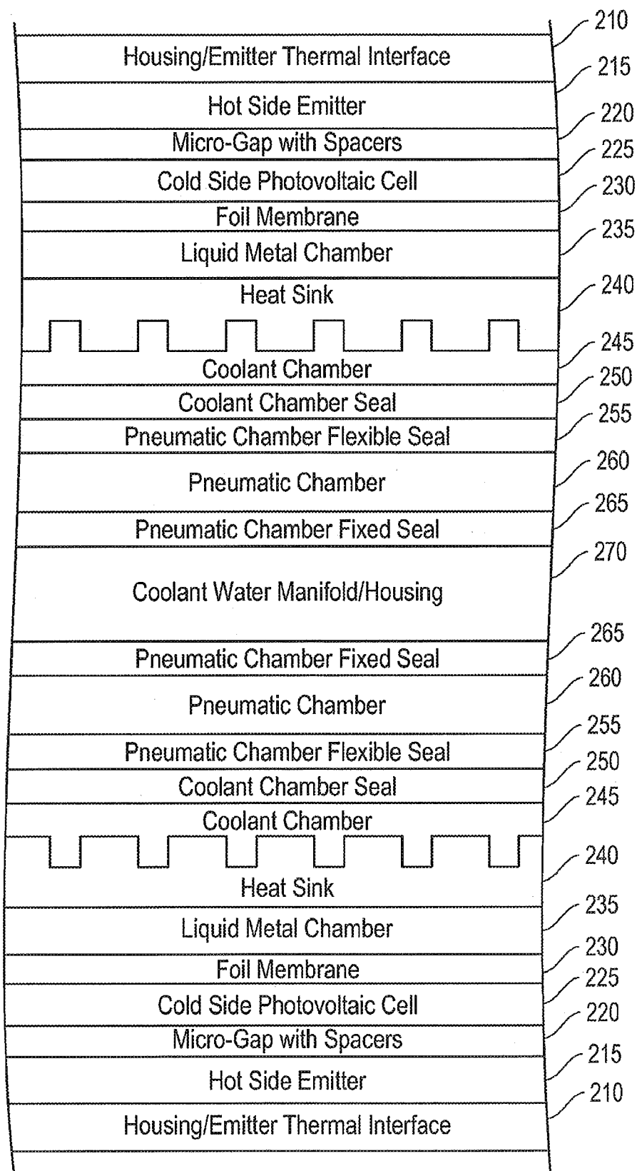
FIG. 2B SUBSTITUTE SHEET (RULE 26)
