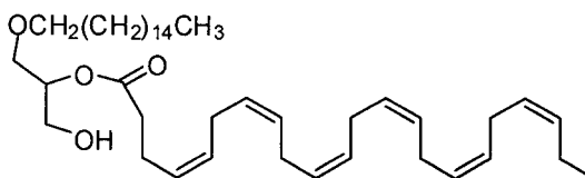
(4Z,7Z,10Z,13Z,16Z,19Z)-1-(hexadecyloxy)-3-hydroxypropan-2-yl docosa-4,7,10,13,16,19-hexaenoate
