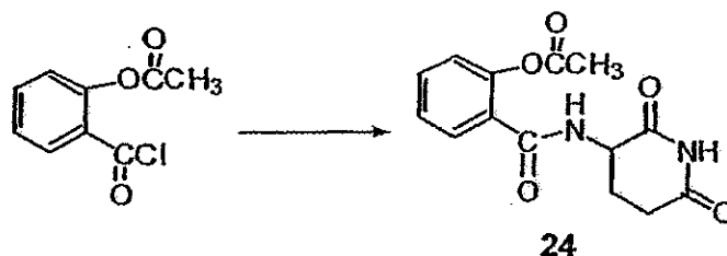
Scheme 10
