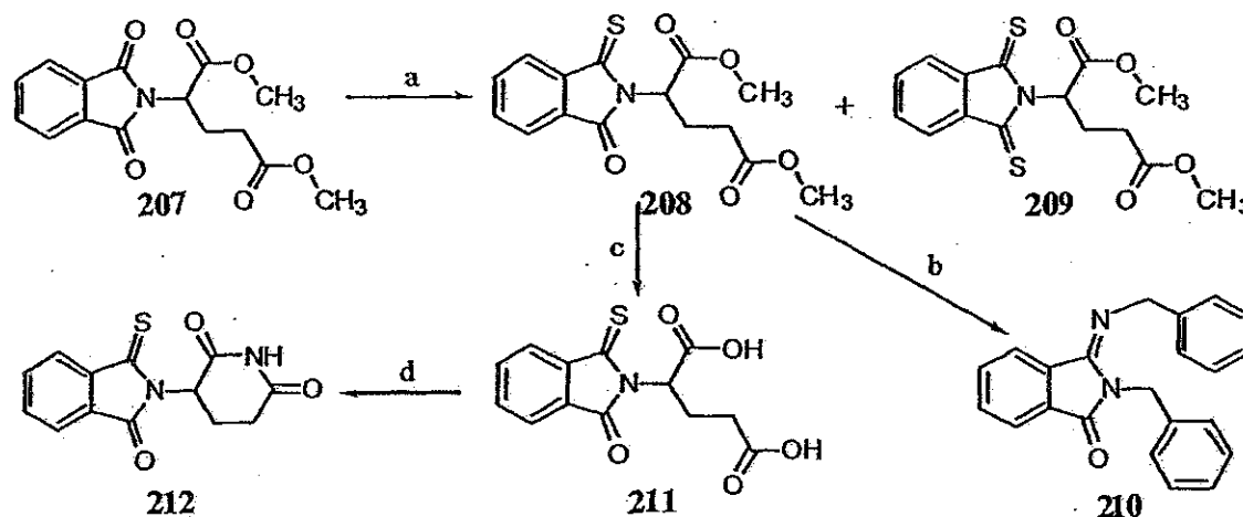
Scheme 12: Reagents: (a) Lawesson's reagent/toluene; (b) Benzylamine; (c) HCl/HOAc; (d) F_3CCONH_2 , HOBt, EDCI, Et_3N/CH_2Cl_2 .
