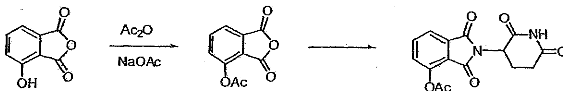
Scheme 5
