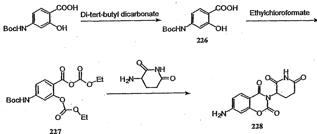
Scheme 17
