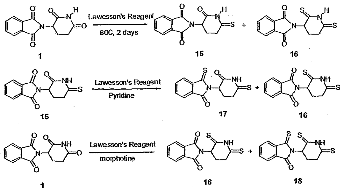
Scheme 7
