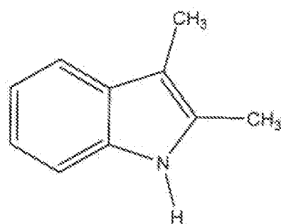
2,3-dimethylindole
