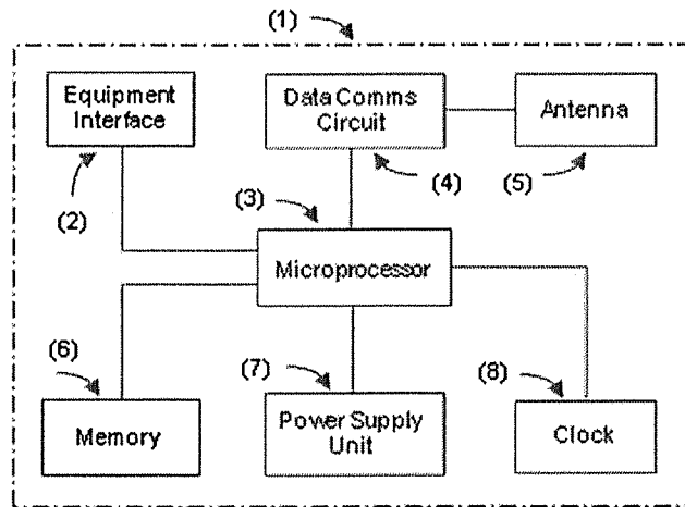
Fig. 1 The invented device
