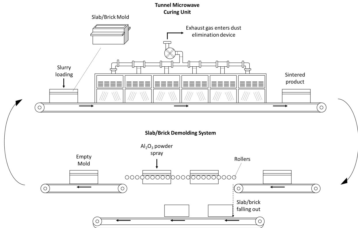
Figure 4: Microwave tunnel curing unit and slab/brick demolding system.
