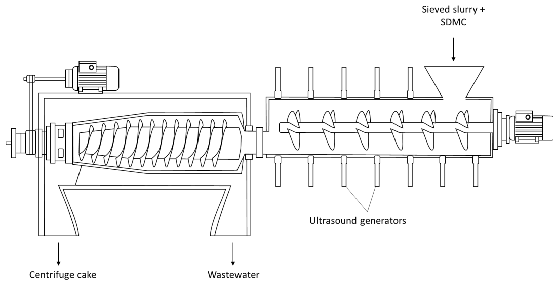
Figure 2: Ultrasonic washing and centrifuge dewatering system.
