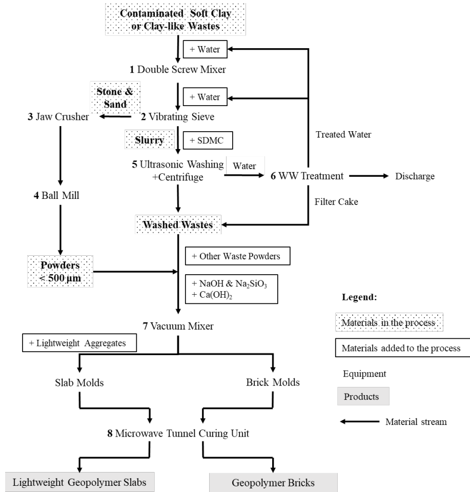
Figure 1: Overview of the soft clay or clay-like waste treatment system.
