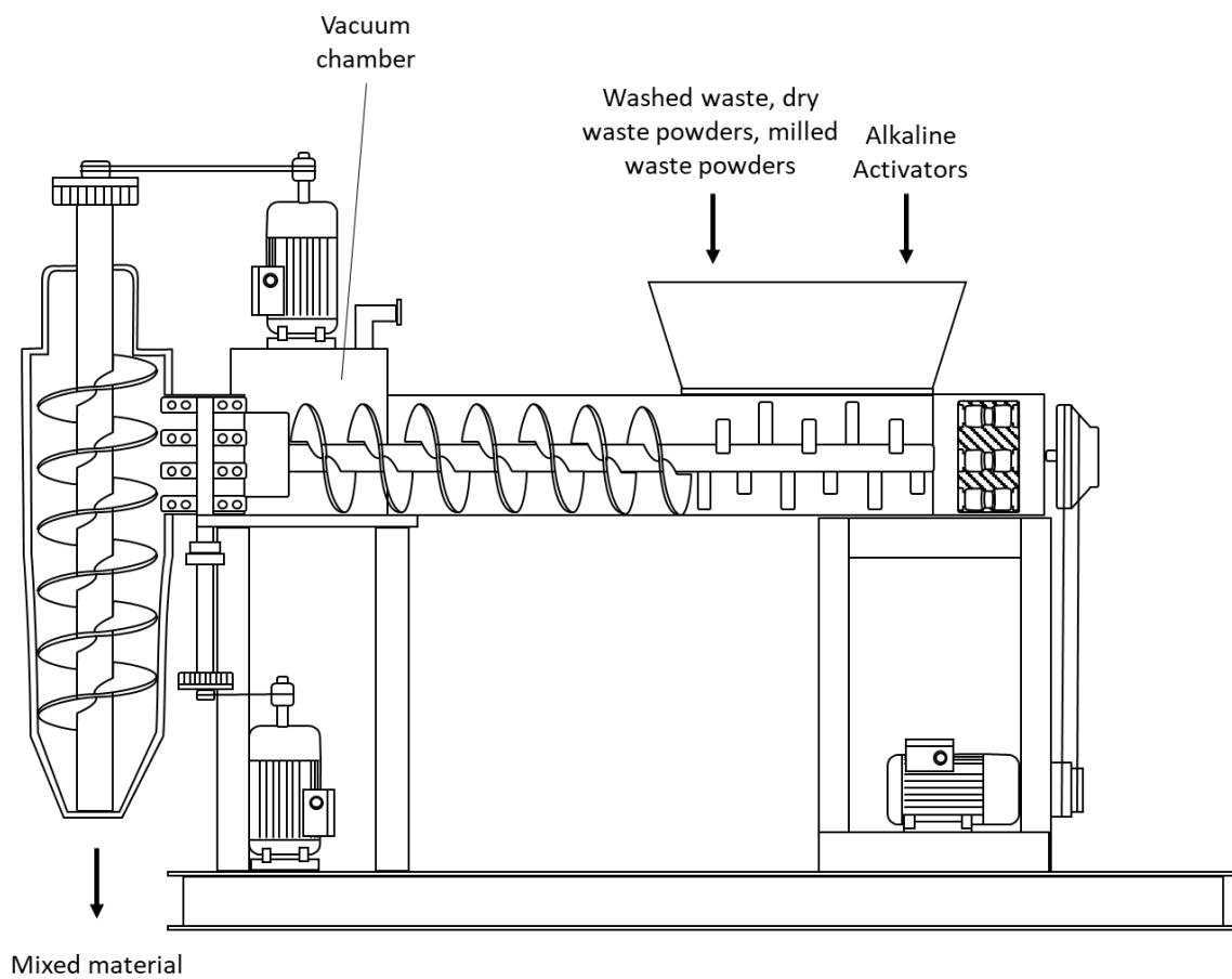
Figure 3: Vacuum mixer system.
