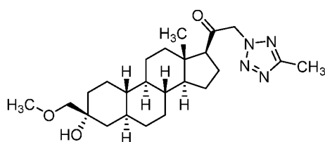
Compound (1).
