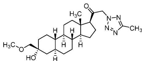
Compound (1), and
