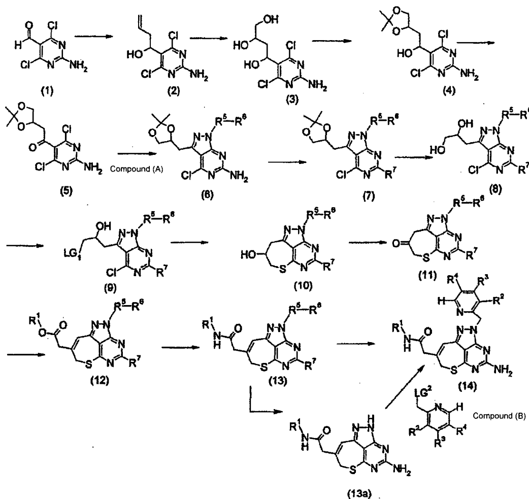
Scheme 1
