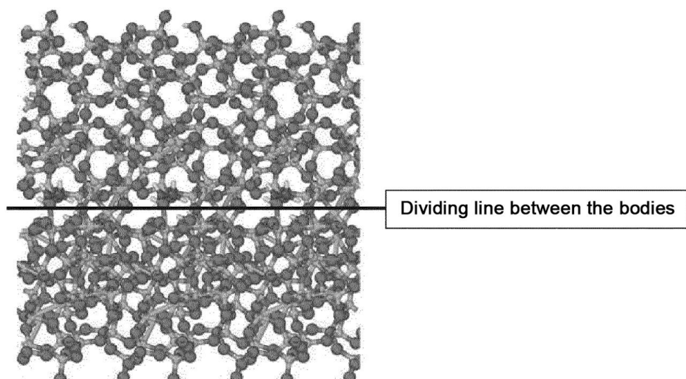
Figure 5 Cold welding of two \text{SiO}_2 surfaces
