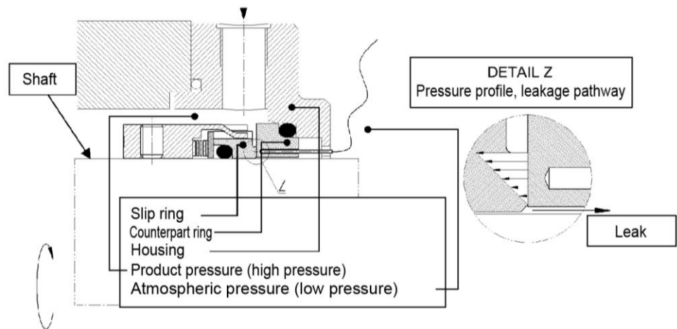
Figure 2 Arrangement of slip ring seal with temperature measurement
