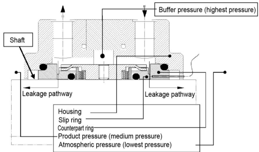
Figure 3 Arrangement of buffered double seal
