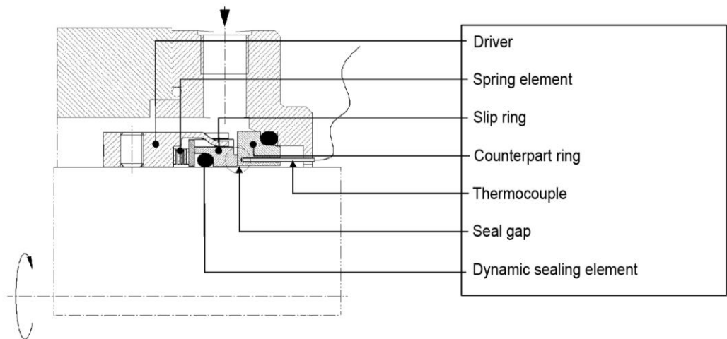
Figure 3 Arrangement of buffered double seal
