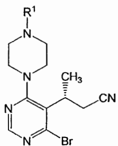
Formula III,
