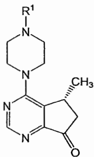
Formula I,
