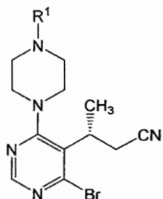
Formula III,
