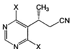
Formula V,
