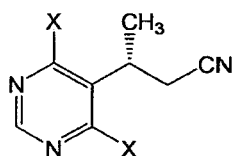
Formula V,
