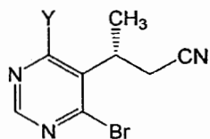
Formula IV,
