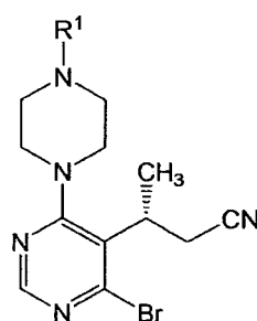
Formula III,
