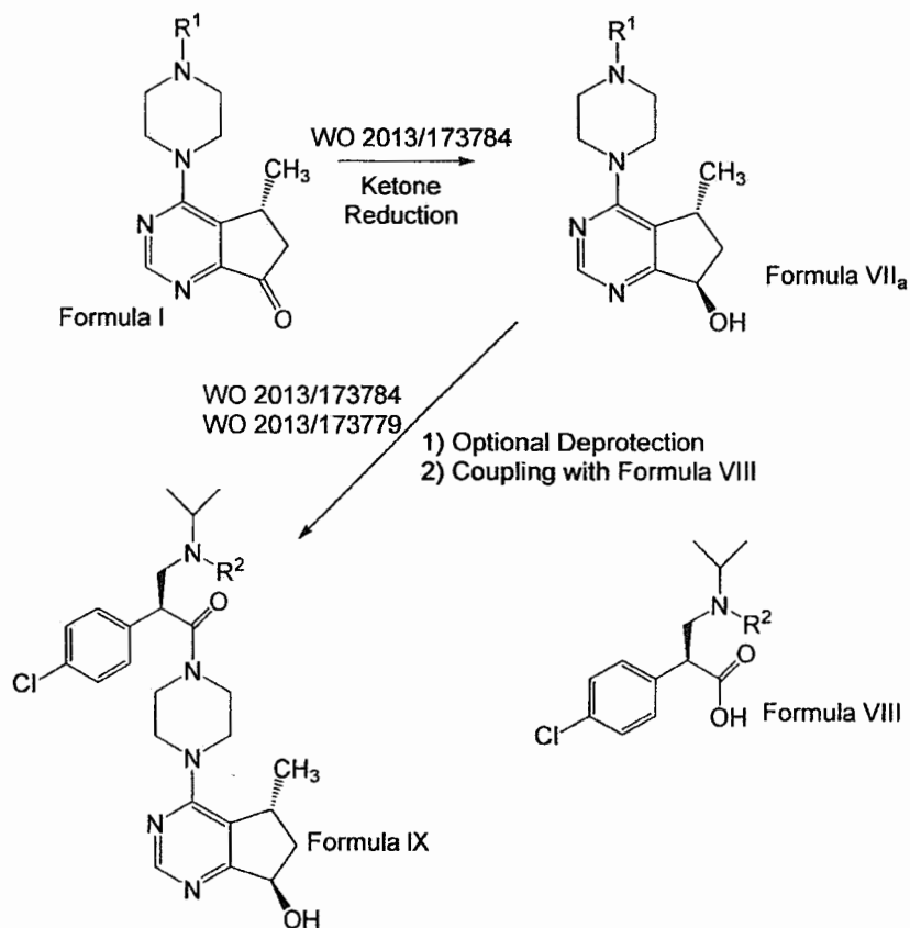
Scheme 5
