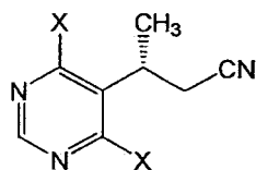
Formula V,
