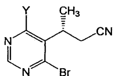
Formula IV,
