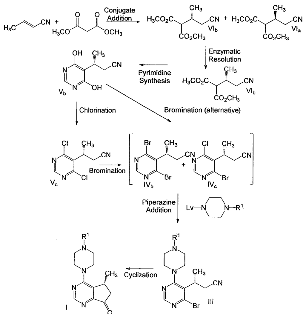
Scheme 3
