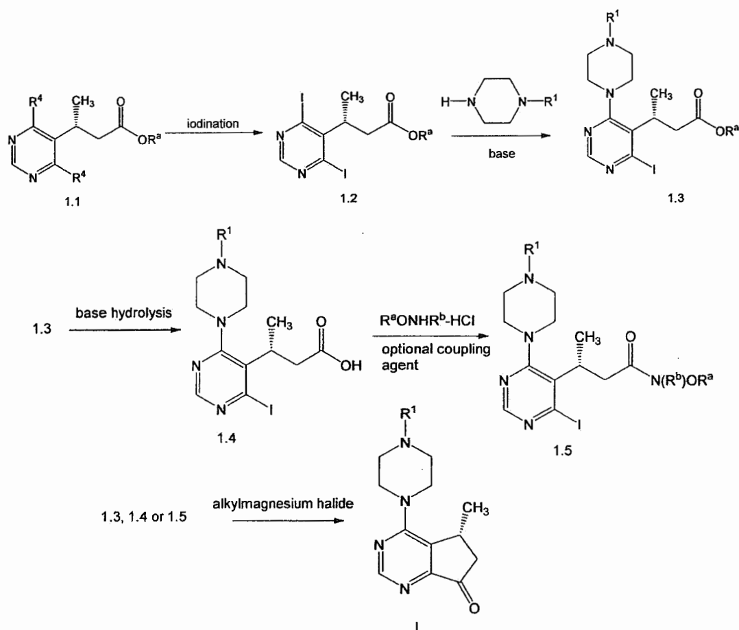
Scheme 1
