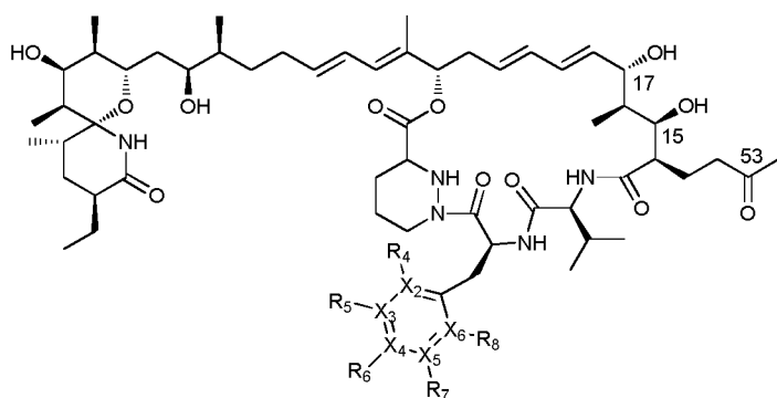
Formula (IIA)
