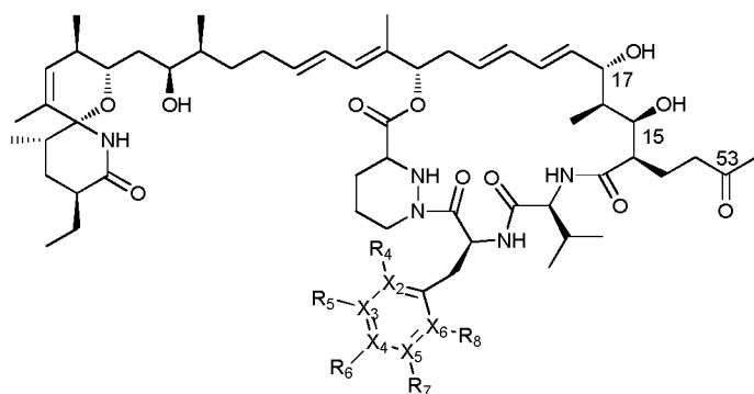
Formula (IIB)
