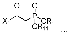
Formula V
