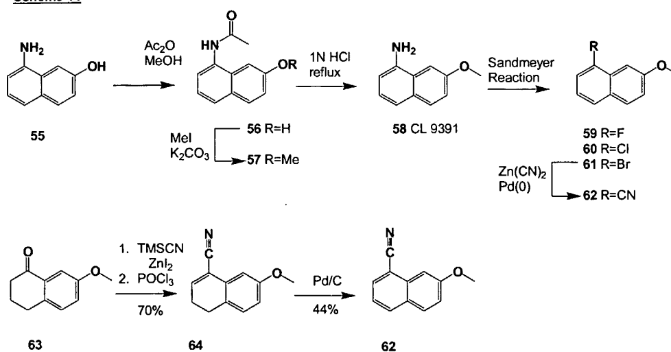
Scheme 11
