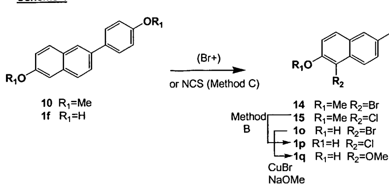
Scheme 4
