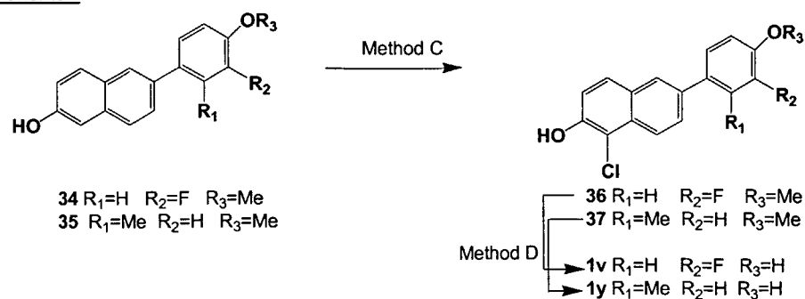
Scheme 7
