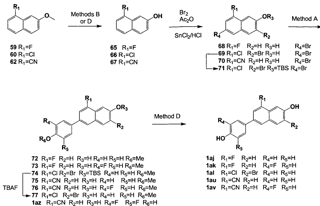
Scheme 12
