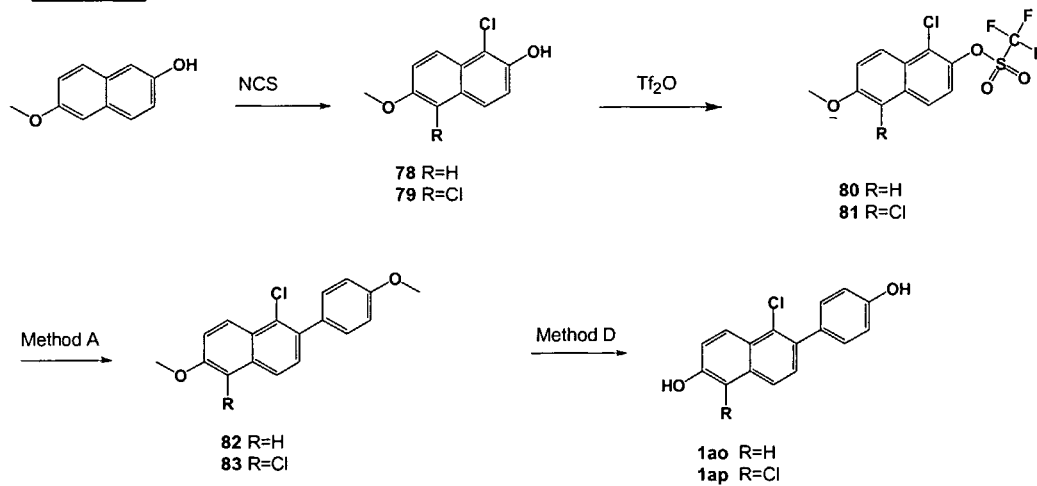
Scheme 13
