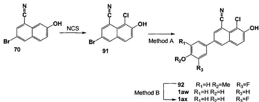
Scheme 15
