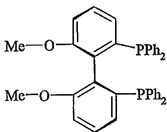
(S)-MeOBiPhep.
