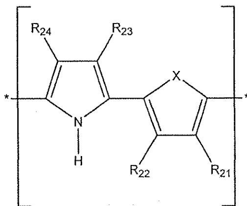
Formula III
