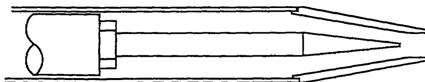
Figure 4. Catalyst spray nozzle enclosed in purging shroud.
