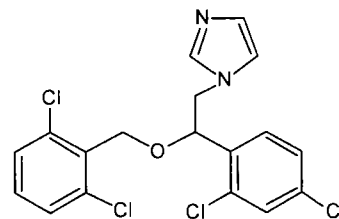
Isoconazole
