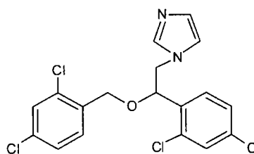
Miconazole
