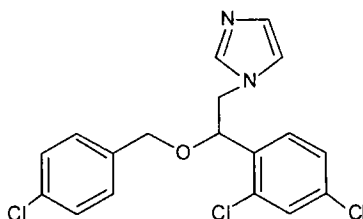
Econazole
