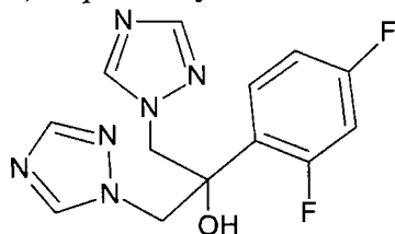
Fluconazole
