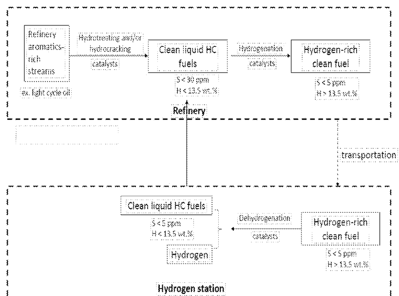
Clean liquid fuels as hydrogen carrier (CLFHC) Process
