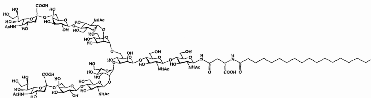
asparagine-linked disialoundecaoligosaccharide-stearic acid amide 5
