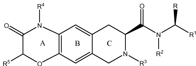
Formula (I-A)
