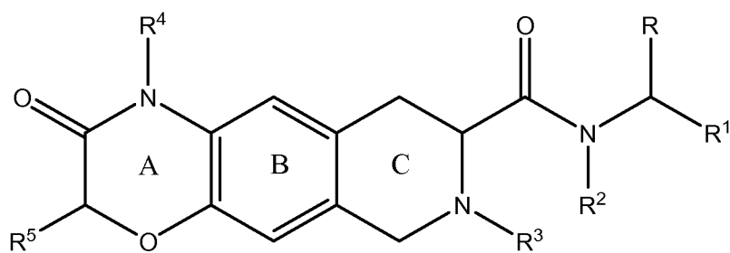
Formula (I)
