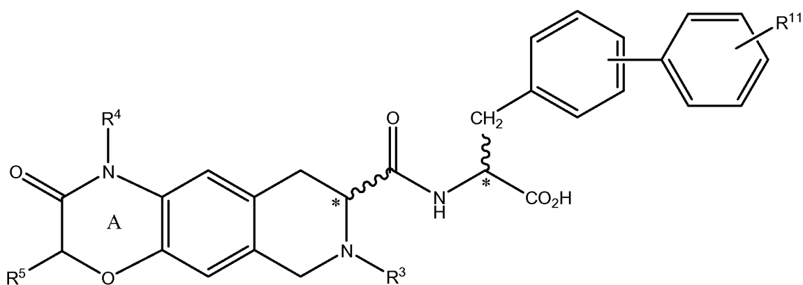
Formula (I-E)
