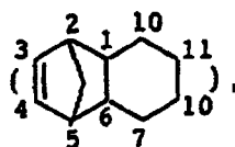
10-methyltricyclo[4,4,0,12,5]-3-undecene, pentacyclo[6,5,1,13,6,0,2,7,0,9,13]-4,10-pentadecadiene
